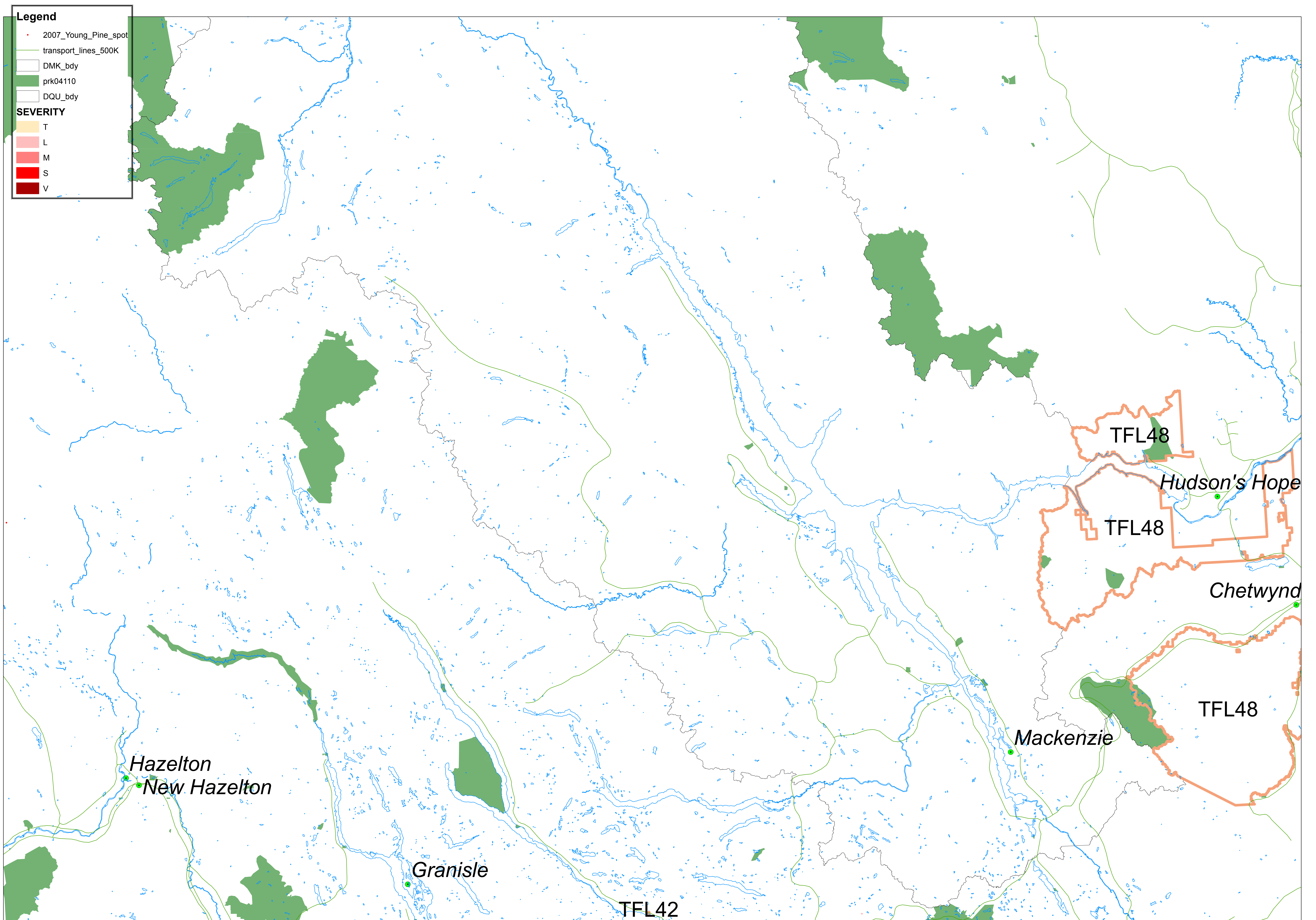
2007 Young Pine Mortality in Mackenzie TSA
